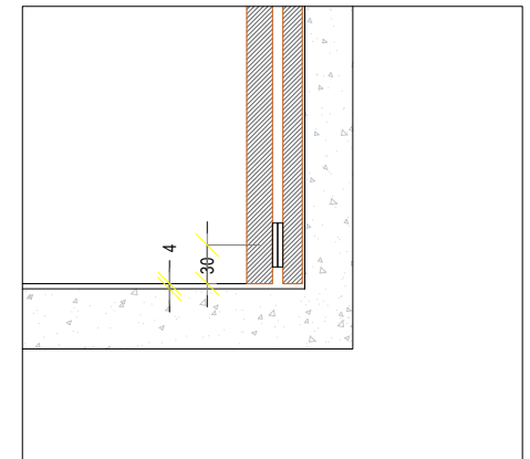
Detail of the vertical section of the wall coating and structure with height from the ground mm 4.
